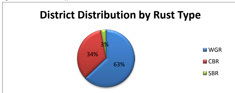
Figure 2.3.1 Nadina Rust Type Distribution
